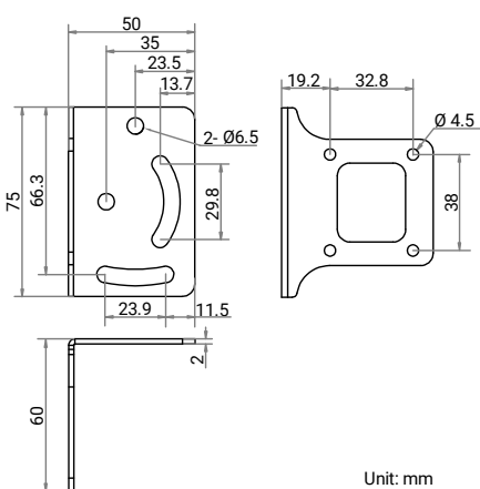
Installation Bracket:
